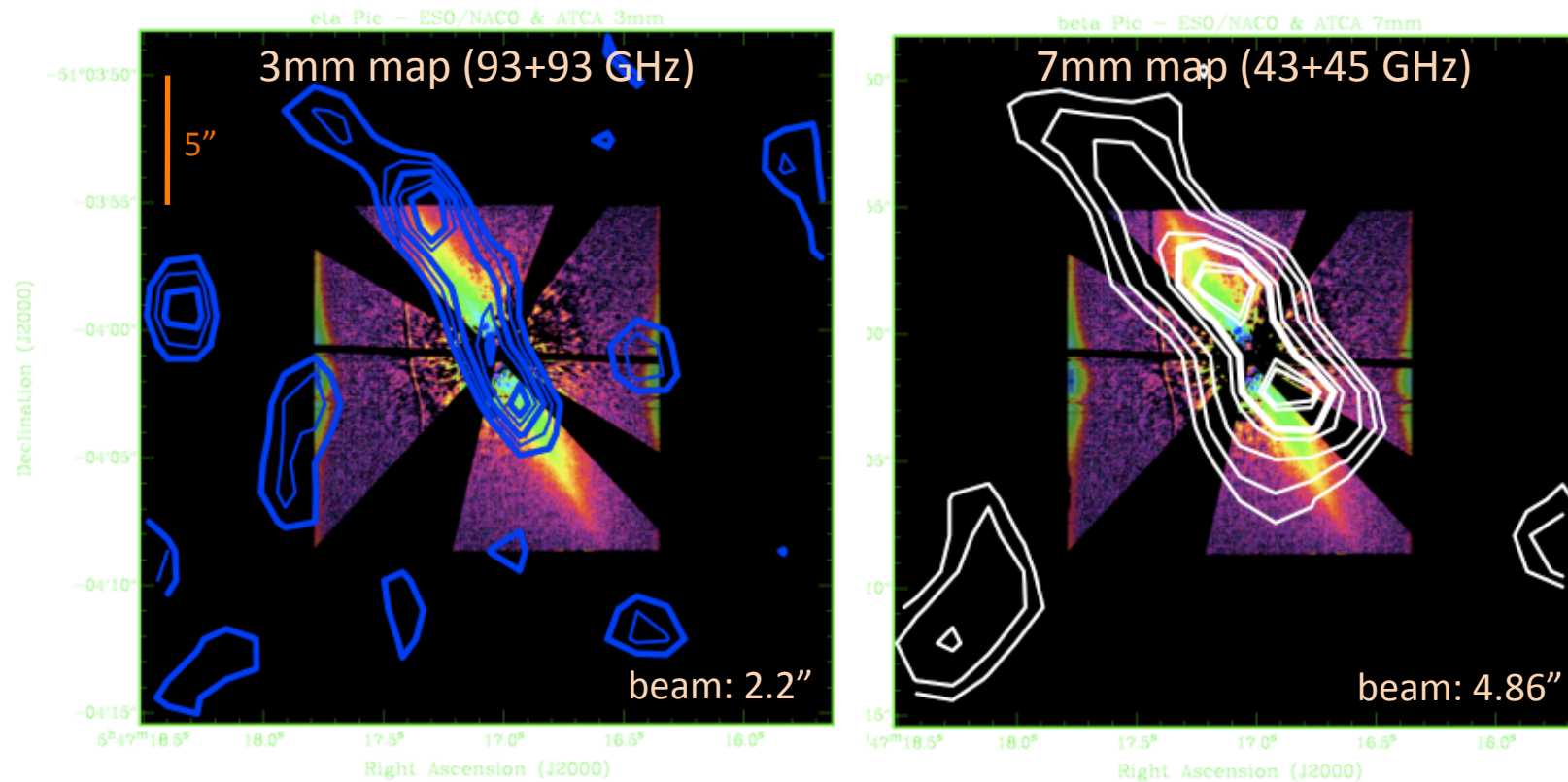
ATCA contours overlaid on ESO/NACO H-band ( 1.65\mu\text{m} ) image (Boccaletti et al. 2009) Lyot chronograph mask ( <0.7'' )
