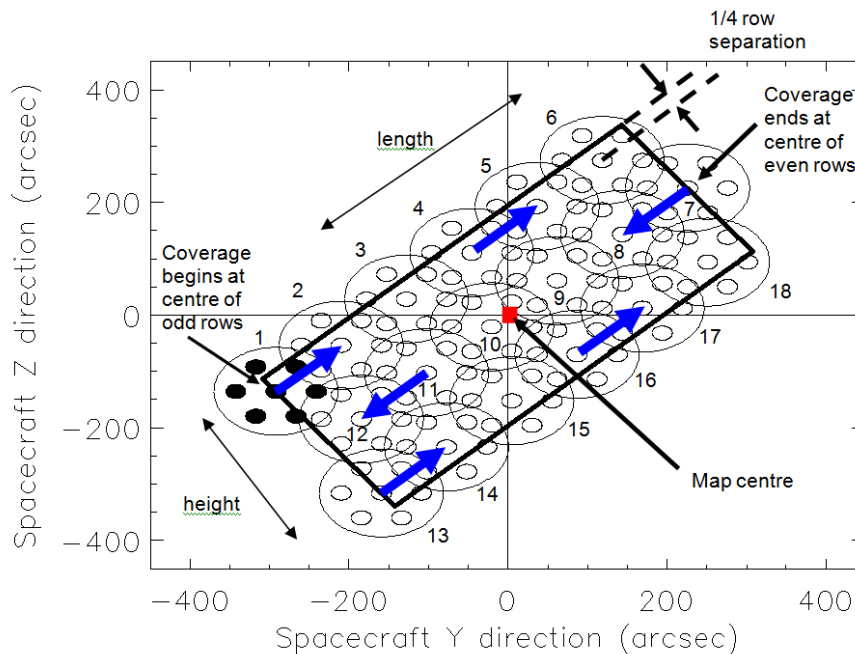
Figure 3.16: Raster map with the SPIRE FTS.
