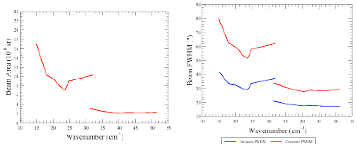
Figure 5.16: Variation of beam FWHM and solid angle across the FTS bands
