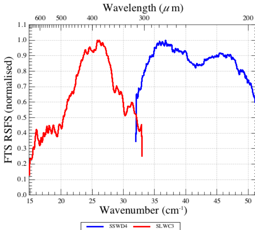
Figure 5.14: The normalised spectrometer RSRF derived for a point source. The two bands have been normalised independently.
