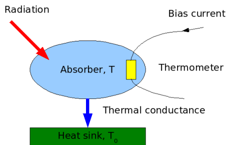
Figure 2.7: Basic principles of bolometer operation.
