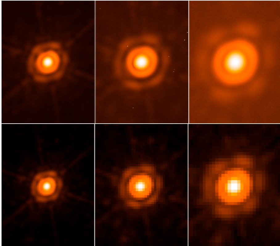
Figure 5.8: Log scale images for the empirical SPIRE beam model at 250, 350, and 500 \mu\text{m} from left to right respectively. The top row uses a 1'' pixel scale for all maps, and the bottom row uses the nominal SPIRE map pixel scales of 6, 10, and 14'' from left to right respectively.
