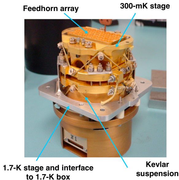
Figure 2.9: Photograph of a SPIRE detector array module.
