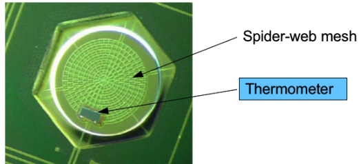
Figure 2.8: Magnified view of a SPIRE bolometer, the thermometer size is 10 \times 100 \times 300 \mu\text{m} .
