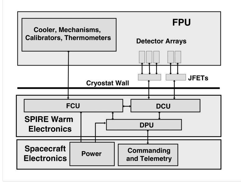
Figure 2.1: SPIRE instrument architecture
