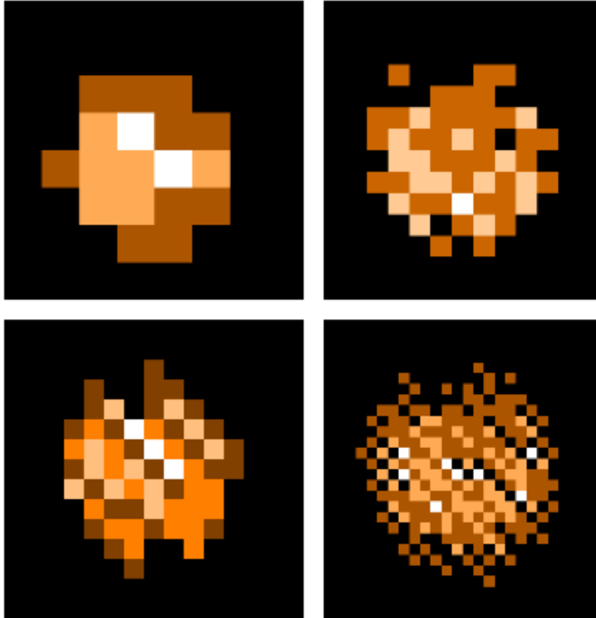
Figure 3.20: Intermediate (top) and Full (bottom) spatial sampling coverage maps for SLW (left) and SSW (right). The sky spectral pixel (spaxel) sizes are 35'' (top left), 17.5'' (bottom left), 19'' (top right), 9.5'' (bottom right). The number of bolometer hits in each sky pixel are encoded with colour. The holes in the maps, due to dead bolometers, depend on the spacecraft attitude (the focal plane position angle), the grid centre, the pixel scale.
