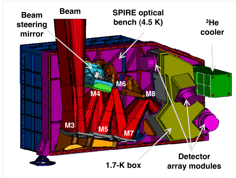
Figure 2.3: SPIRE FPU: photometer side layout.
