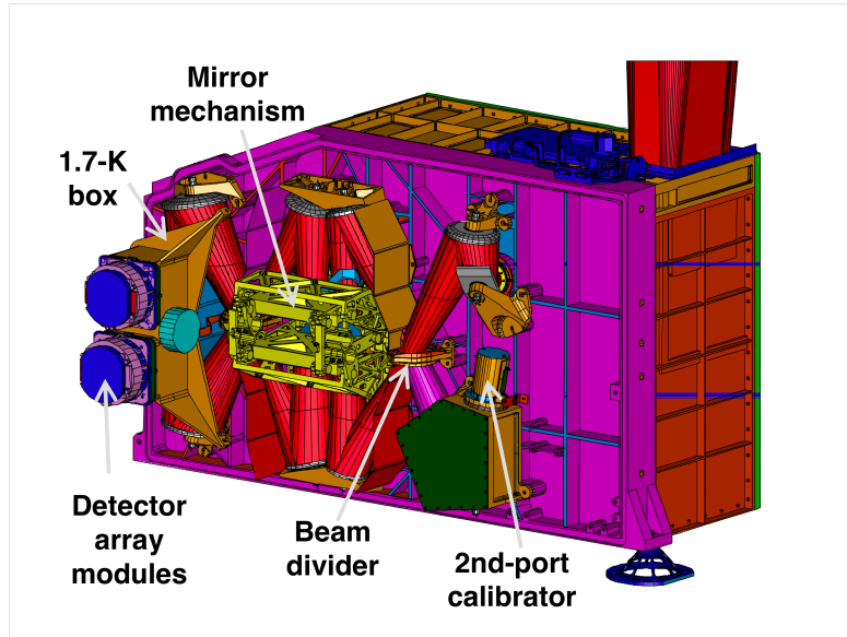
Figure 2.5: SPIRE FPU: spectrometer side layout.
