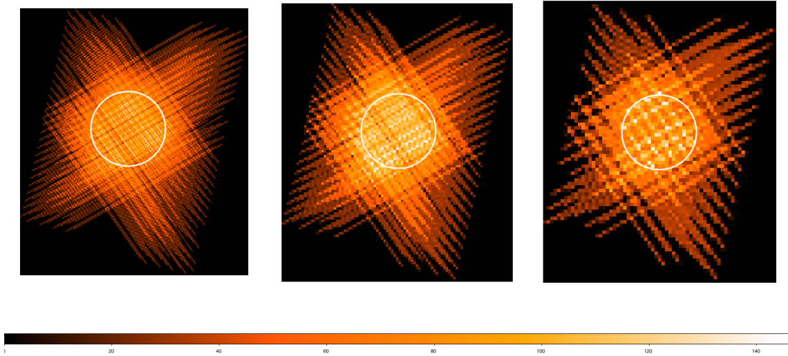
Figure 3.8: Example coverage maps for Small Map mode for the three photometer arrays, PSW (left), PMW (centre) and PLW (right). The white circle is with 5 arcmin diameter. The pixel size is (6",10",14") for (PSW, PMW, PLW) and the colour code represents the number of bolometer hits in each sky pixel.
