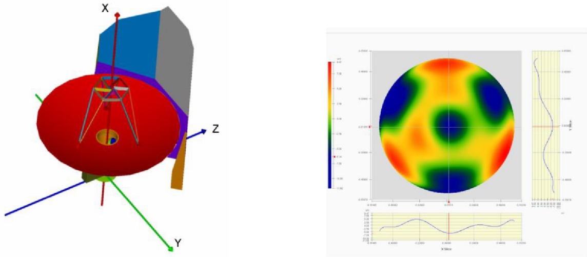
Figure 5.10: View of the model geometry (left) and reconstructed telescope pupil optical path difference map from environmental ground measurements by Herschel Observatory industrial contractors (right).
