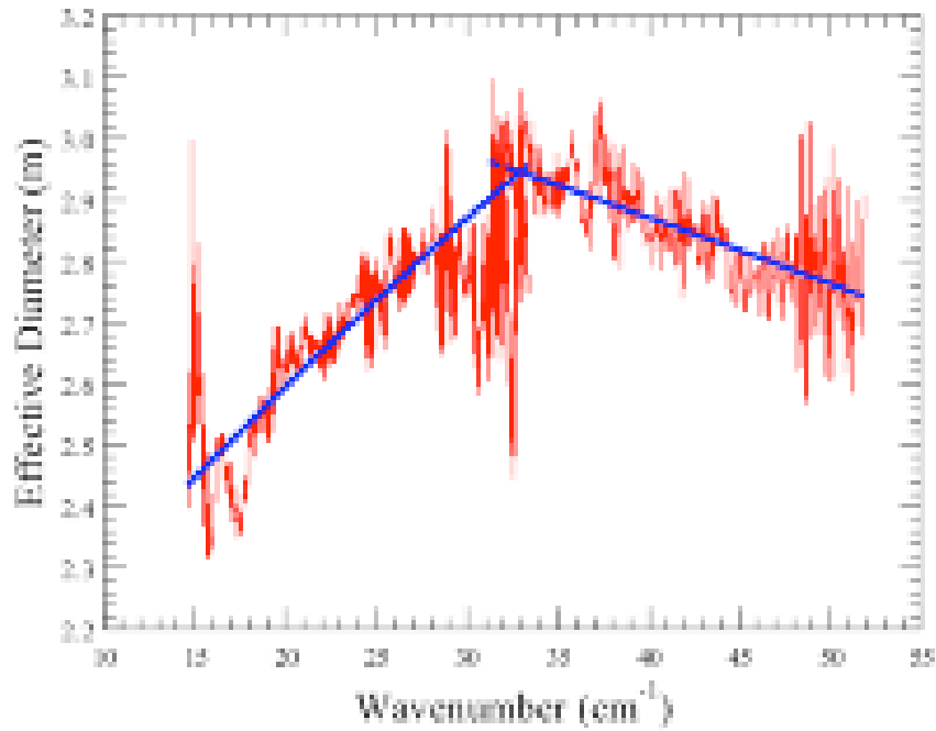
Figure 5.15: Effective telescope diameter vs. wavenumber
