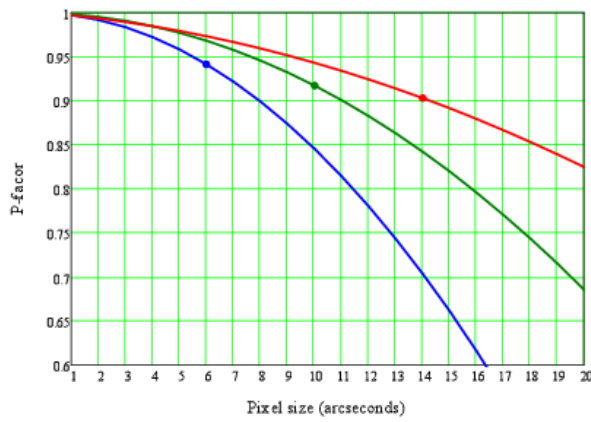
Figure 5.13: Map pixel size correction factor vs. pixel size for the SPIRE photometer bands: 250 \mu\text{m} (blue), 350 \mu\text{m} (green), 500 \mu\text{m} (red). The dots indicate the standard SPIRE Level-2 map pixel sizes.
