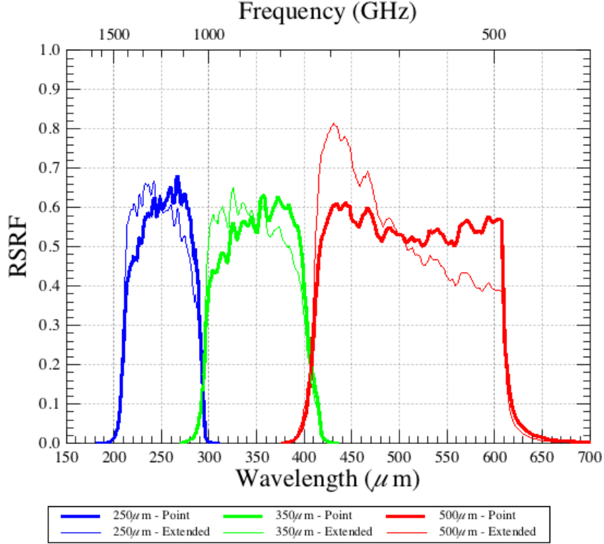
Figure 5.5: Photometer RSRFs: R_P(\nu) (thick lines; point source; no weighting of filter transmission profiles) R_E(\nu) (thin lines; extended source; \lambda^2 weighting).
