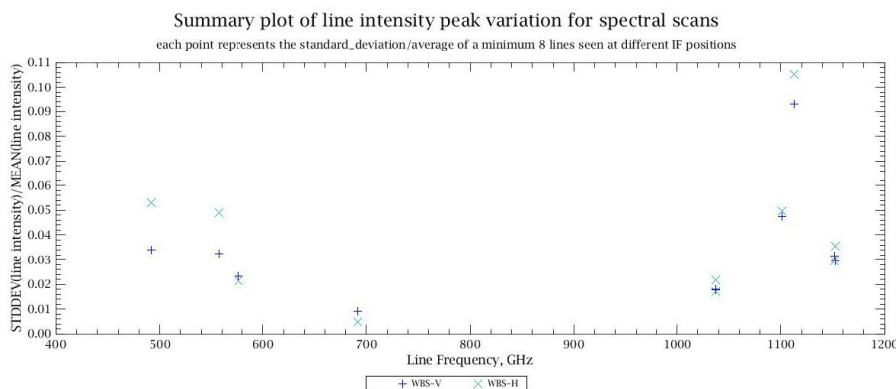
Figure 5.19. Peak intensity variation of spectral lines as measured at 8 or more positions in the IF, from performance verification Spectral Scans..
