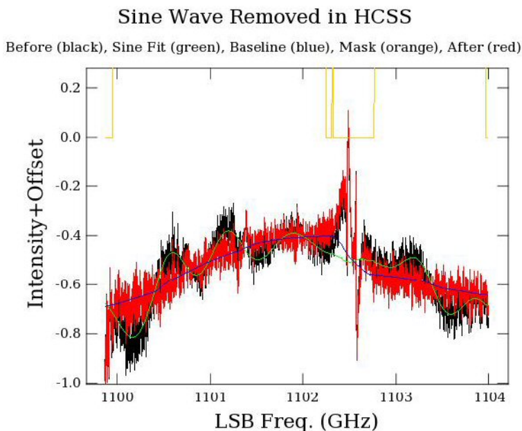
Figure 4.11. Band 4b observation using Point Frequency Switch, showing a strong residual standing wave (black). Its period ( \sim 600 MHz) and increasing amplitude toward the band edges are those expected for diplexer bands. It was fitted with a combination of sine waves using FitHifiFringe (green). The corrected spectrum (red) still shows a strongly curved baseline that can be subtracted with a polynomial fit in HIPE.
