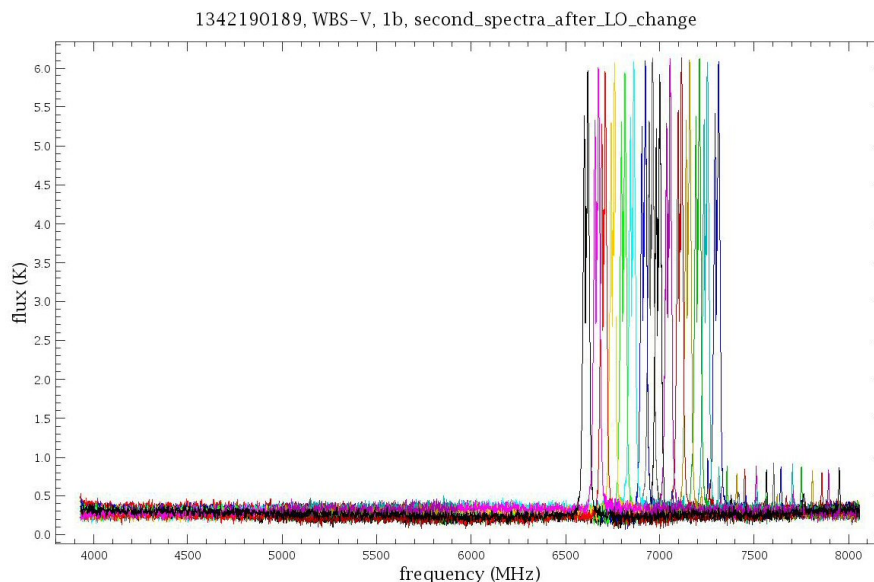
Figure 5.17. CO 5-4 for NGC 7538 IRS 1 with WBS-V, spaced across the upper sideband from an engineering Spectral Scan.
