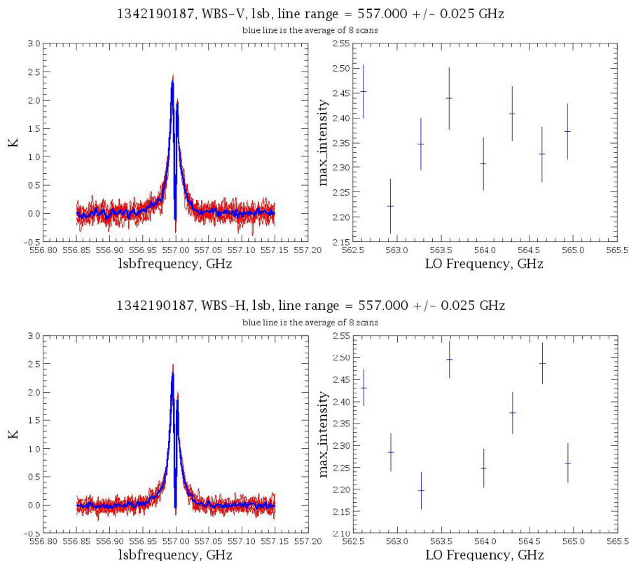
Figure 5.18. Measurements of the 557 GHz water line at 8 positions in the LSB in WBS-V (upper) and WBS-H (lower).
