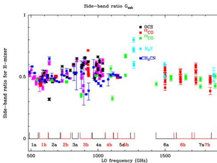
Figure 5.16. Measured side-band ratio from on-ground gas cell measurements
