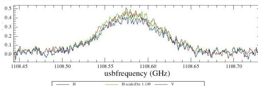
Figure 5.7. Line profile of NML Tau at 1108.5 GHz. H and V profiles in this observation differ by 26% at the peak, rescaling so the peaks match show no difference in line shape
